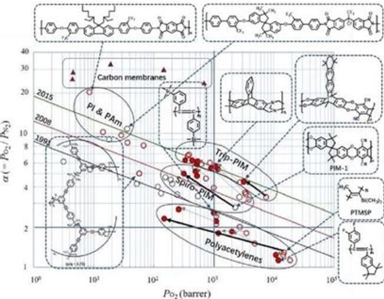
Upper plots through polymers showing the highest \alpha at each P_{O_2} reported in the literature in 2020 (●: after aging, ○: before aging).
