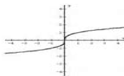
f(x) = \sqrt[3]{x} Cube Root
