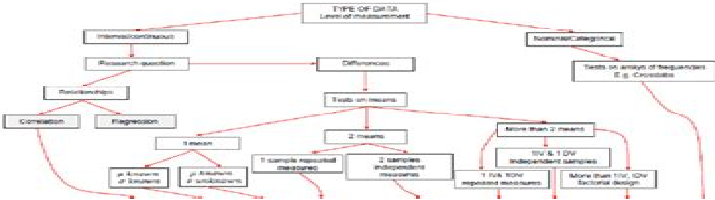
STATISTICAL ANALYSIS DECISION-MAKING TREE
