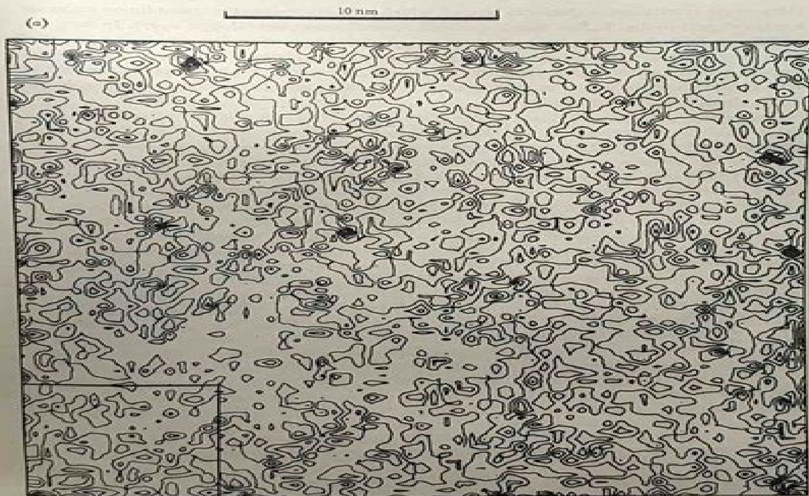
FIGURE 12. Difference image of an amorphous carbon foil, 10 to 20 nm thick. The two original micrographs were registered with the same electron optical parameters ( \lambda = 3.7 pm, C_s = 3.9 mm; x_s = 410 nm, \Delta f_s = 124 nm) at a magnification of 180 000 on photographic films. The difference image shows the change of the foil after an electron bombardment of 80 000 to 110 000 electrons per square nanometre in the microscope. The total pressure of the residual gases in the microscope (Elmiskop 1a) was about 10^{-6} Torr ( 13 \mu\text{N m}^{-2} ); the specimen was surrounded by a chamber cooled down to liquid nitrogen temperatures. In (a) the difference between two successive lines of equal intensity corresponds to a step \Delta S = 0.05 of the registered optical density; lines of positive and negative values are not distinguished. The resolution of the map is 0.45 nm, i.e. for mapping all Fourier coefficients with d^* = (1/d) > (1/0.45 \text{ nm}) were set to zero. In the lower corner on the left of figure 12a the region is marked which is shown in figure 12b in more detail: resolution 0.3 nm, difference between two successive lines of equal optical density \Delta S = 0.03 . High maxima are marked by the symbols A 0, A 1, ..., E 9, A 0 denoting the highest value and so on; low minima are marked by the symbols V 0, V 1, ..., Z 9, starting with the lowest value V 0. (c) finally shows the reconstructed difference image of (b) using the same contour level distances as in (b).
