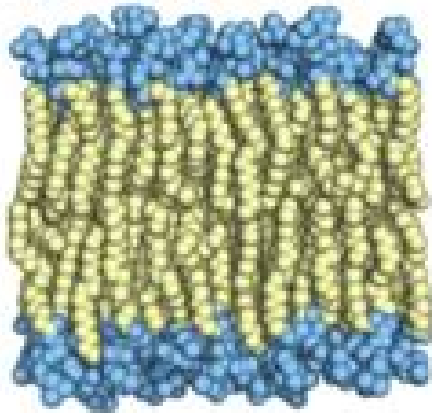
(a) Liquid-ordered state L_o
