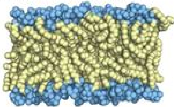
(b) Liquid-disordered state L_d
