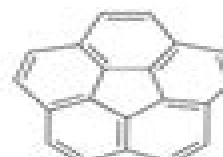
Coranulene
