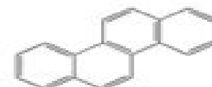
Chrysene
