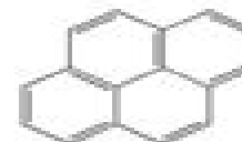
Pyrene
