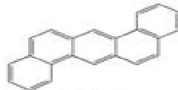
Dibenz(a,h)anthracene
