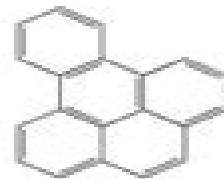
Benzo[e]pyrene
