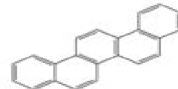
Picene
