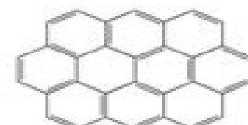
Ovalene
