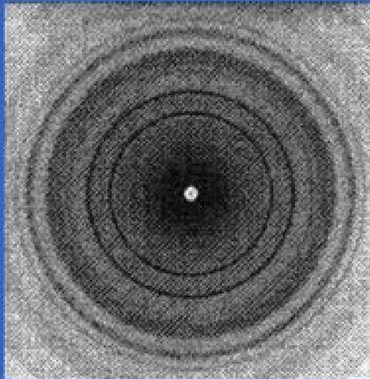
semicrystalline poly(3-hydroxybutyrate)
