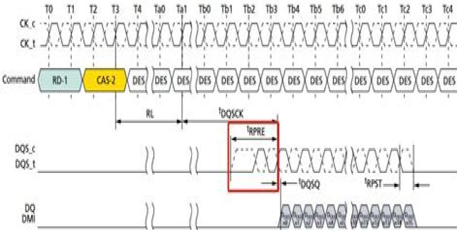
Figure 13: DQS Read Preamble and Postamble - Toggling Preamble and 0.5nCK Postamble
