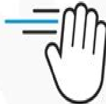
Gesture-based Interfaces
