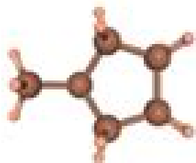
BN-methylcyclopentane
