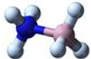
\text{NH}_2\text{BH}_3
