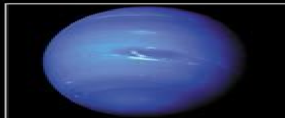
Neptune
