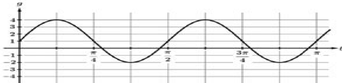
Graph of g
