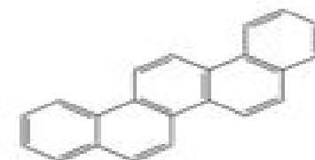
Picene
