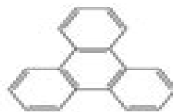
Triphenylene
