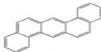
Dibenz(a,h)anthracene
