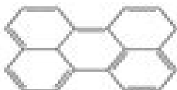
Perylene
