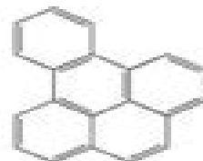
Benzo[e]pyrene
