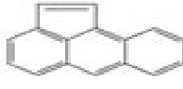
Aceanthrylene
