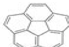
Coranulene
