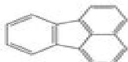
Fluoranthene
