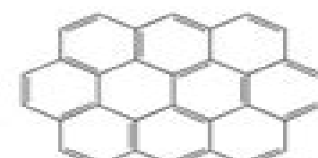
Ovalene
