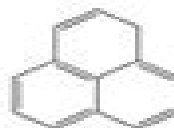
Phenylene
