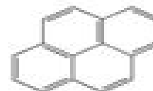
Pyrene
