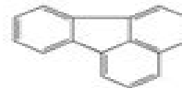
Fluoranthracene
