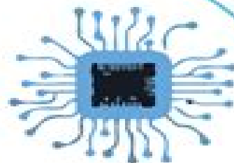
Machine Learning
