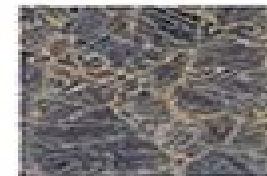
Anorthosite p (brown), py, b
