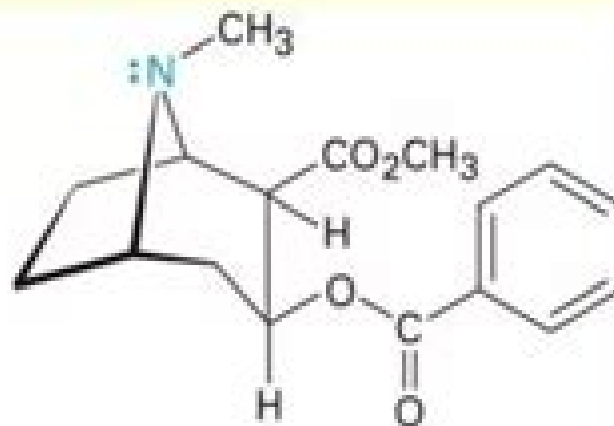
Cocaine
