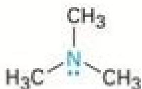
Trimethylamine
