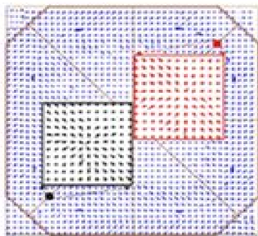
Minimum number of WPs
