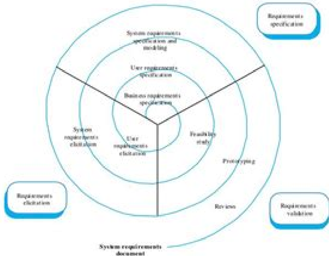
Figure 7.2 Spiral model of requirements engineering processes
