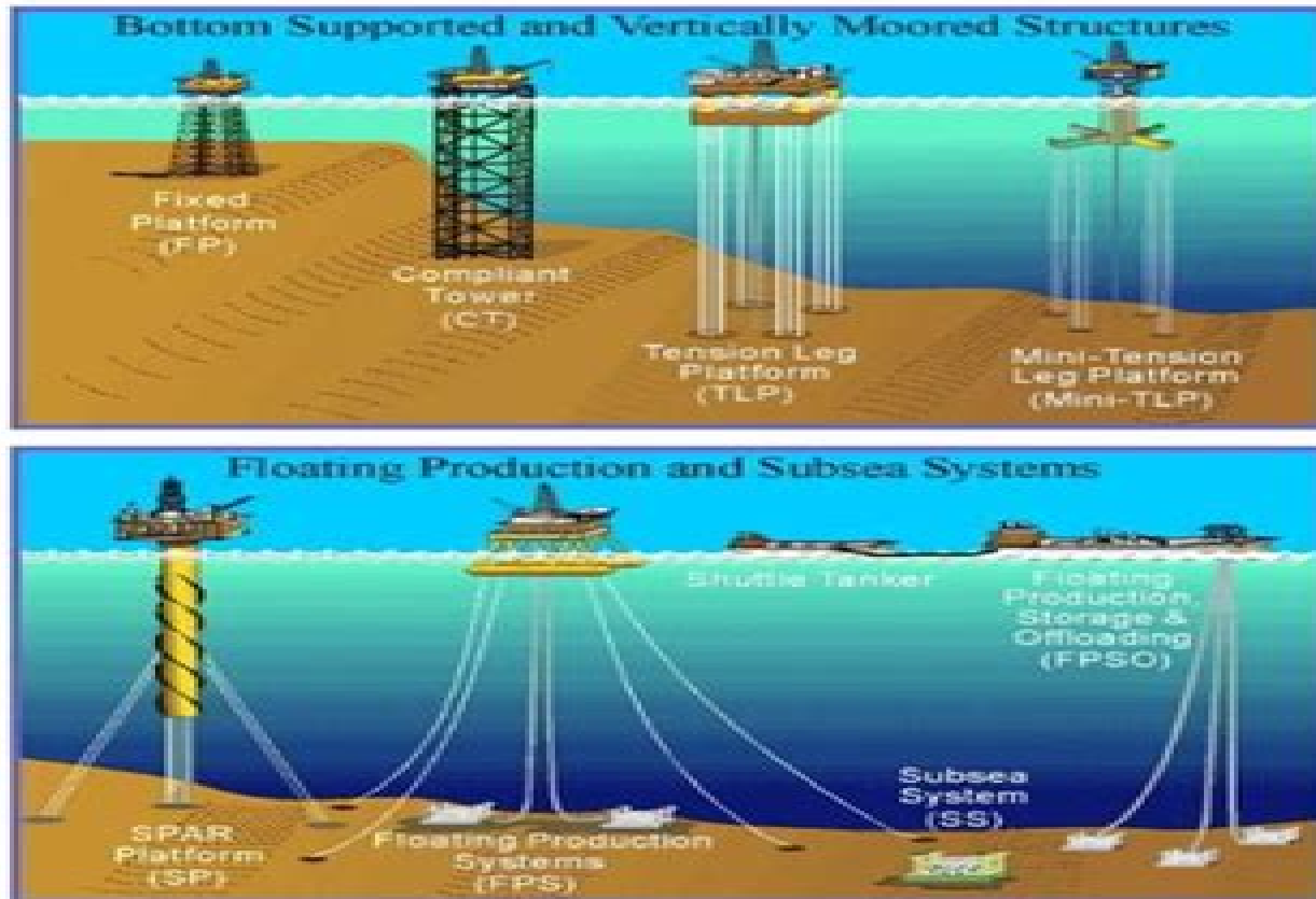
Figure 1.1: Different types of Offshore Structures
