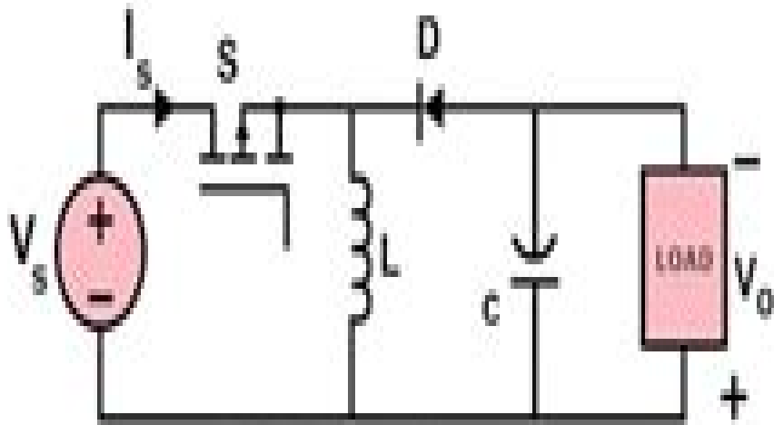
Buck-Boost Converter
