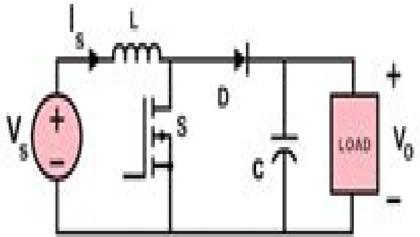
Boost Converter
