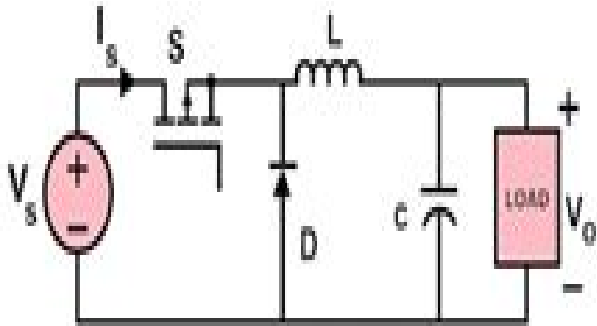
Buck Converter
