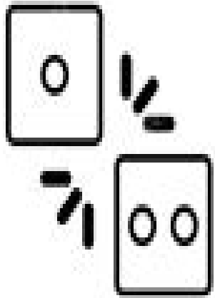
Probability
