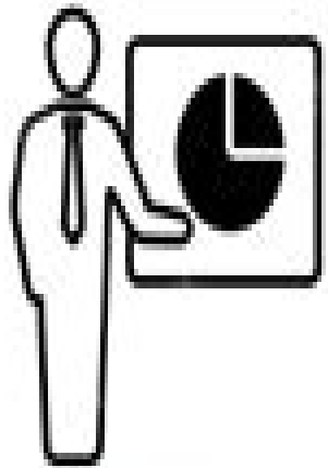
Statistician
