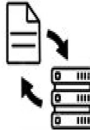
Data Collection
