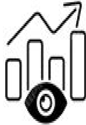
Prediction
