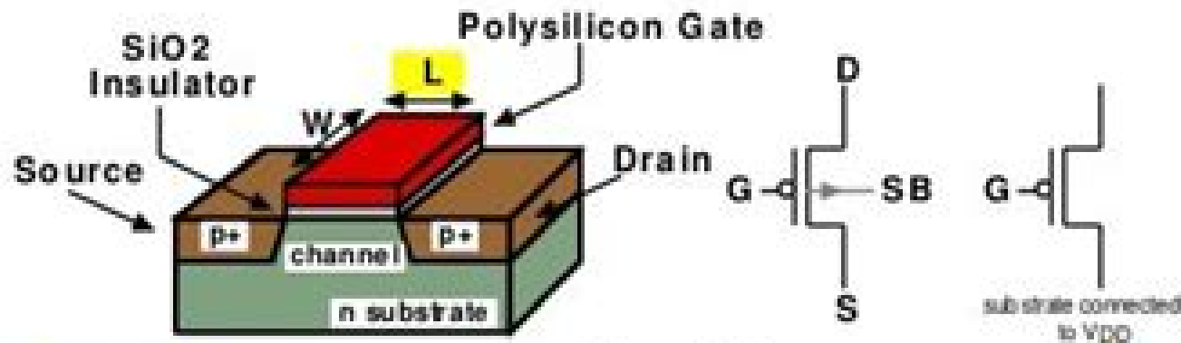
p transistor
