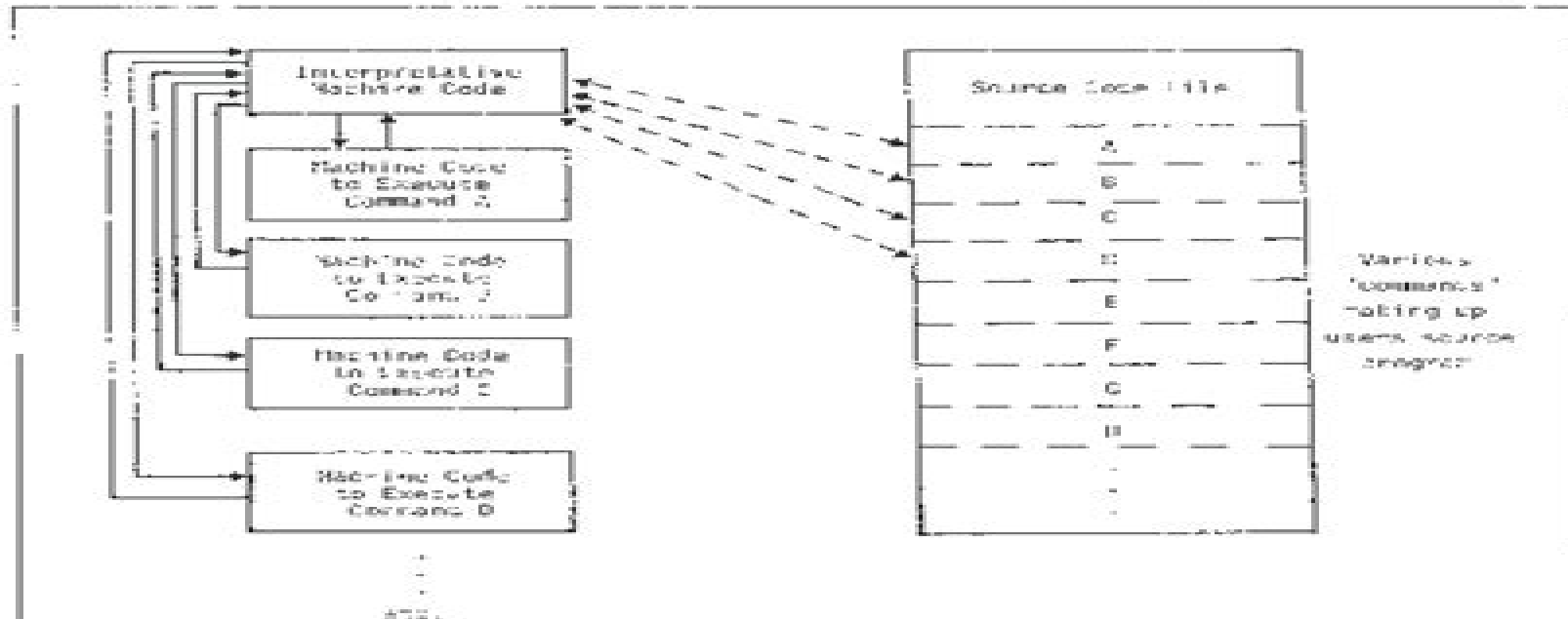
Figure 1. The interpretative cycle of common parts of languages such as BASIC. After assembly, each command in the source file, the interpreter generates for each line of the corresponding block of machine code then, program execution always resumes within the interpreter.
