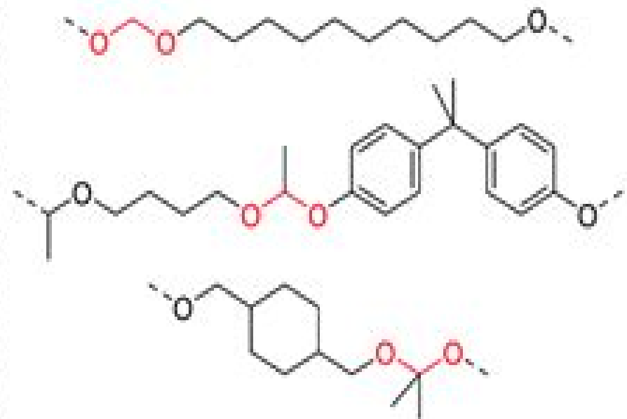
polyacetals with linear acetal units
