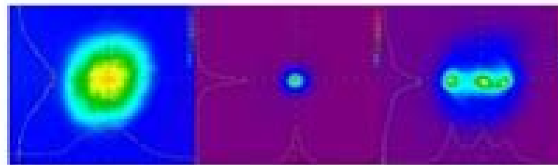
Soliton generation and modulation instability
