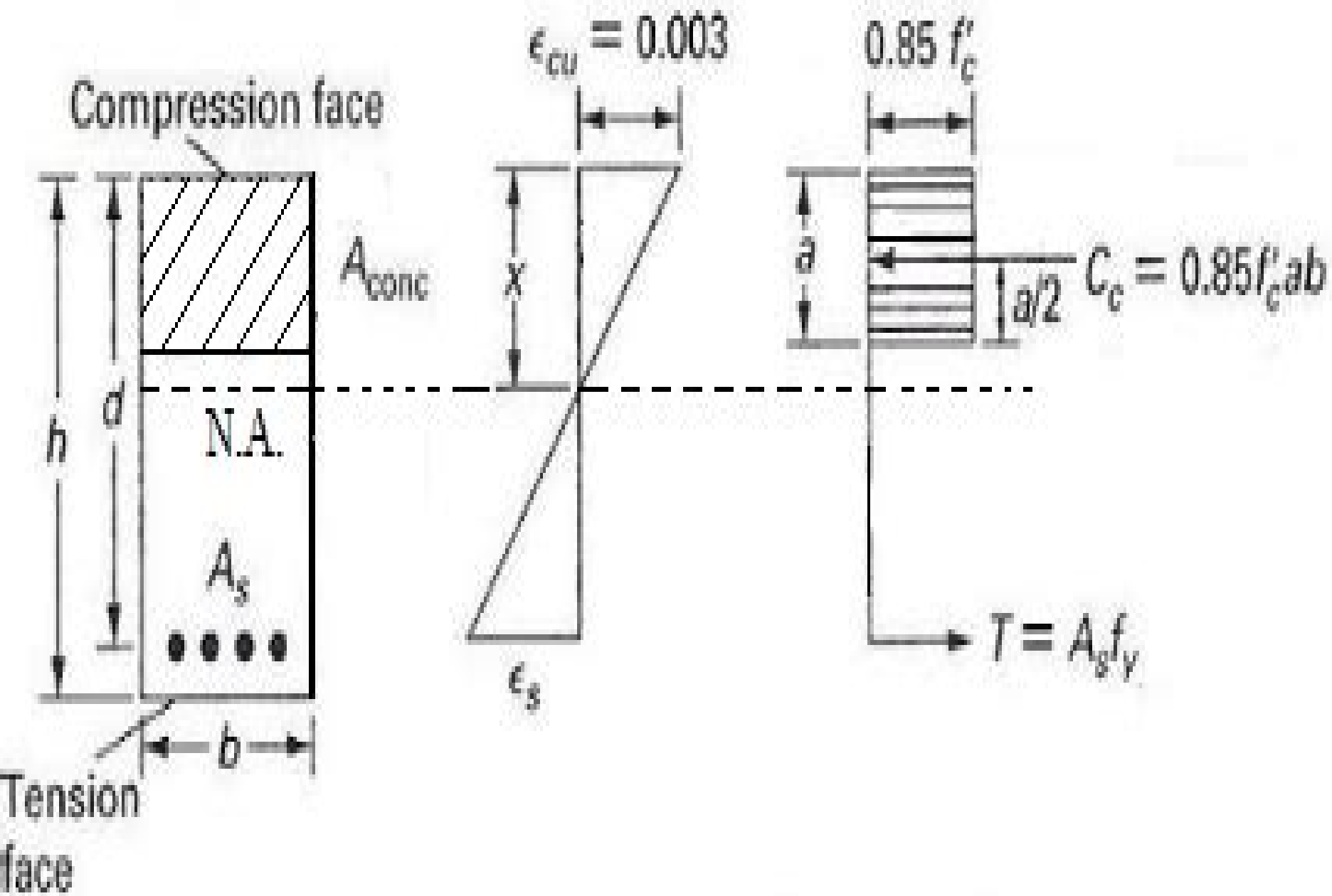
(c) Stress diagram
