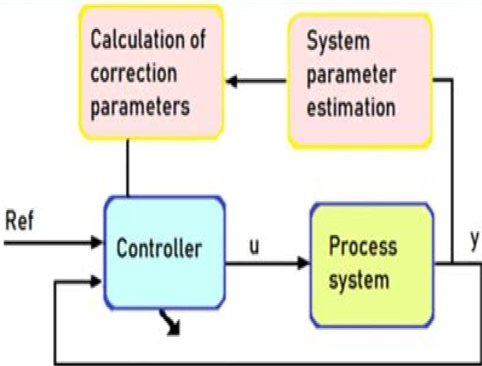
Indirect Adaptive Control Scheme
