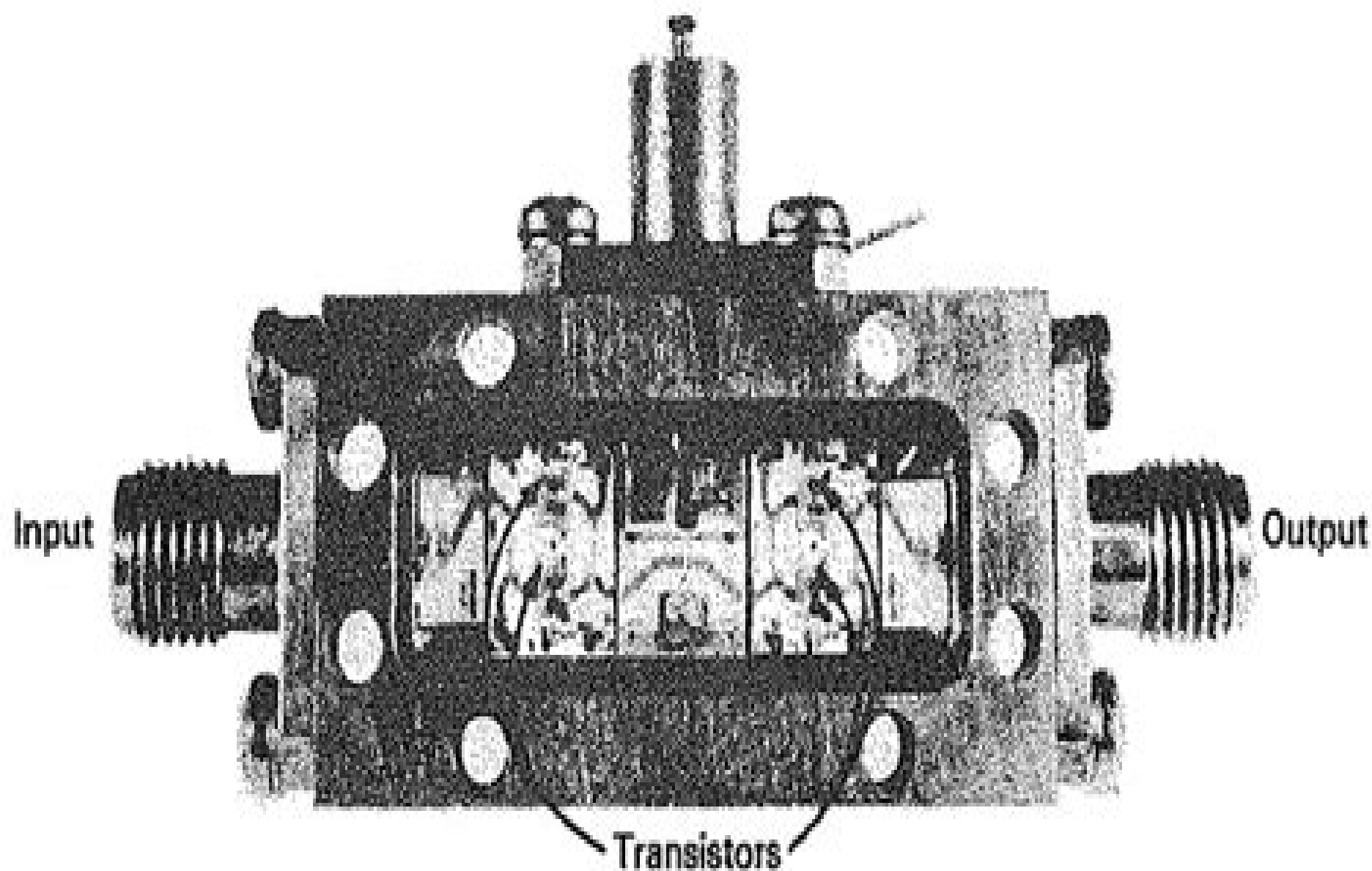
FIGURE 12-6 Hybrid GaAs FET MIC amplifier. Note: Hermetically sealed cover removed.
