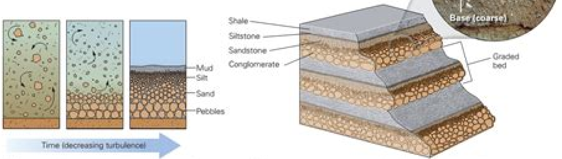
(b) As the turbidity current slows, larger grains settle first, followed by progressively finer grains.
