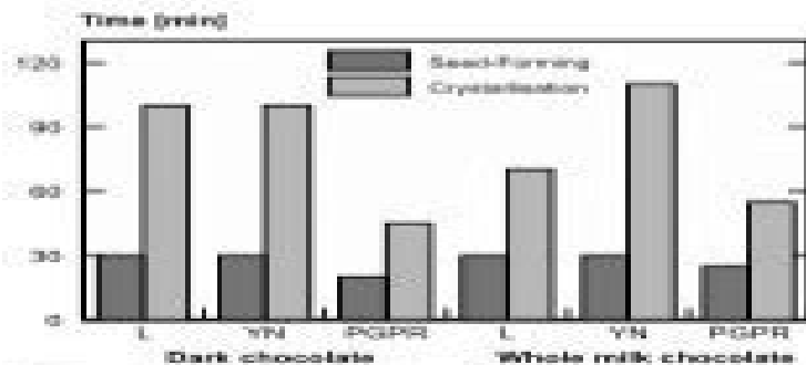
Figure 3: Seed-forming time and crystallisation time of chocolate masses as affected by the emulsifier. L, lecithin; YN, ammoniumphosphate; PGPR, polyglycerol polyricinoleate.
