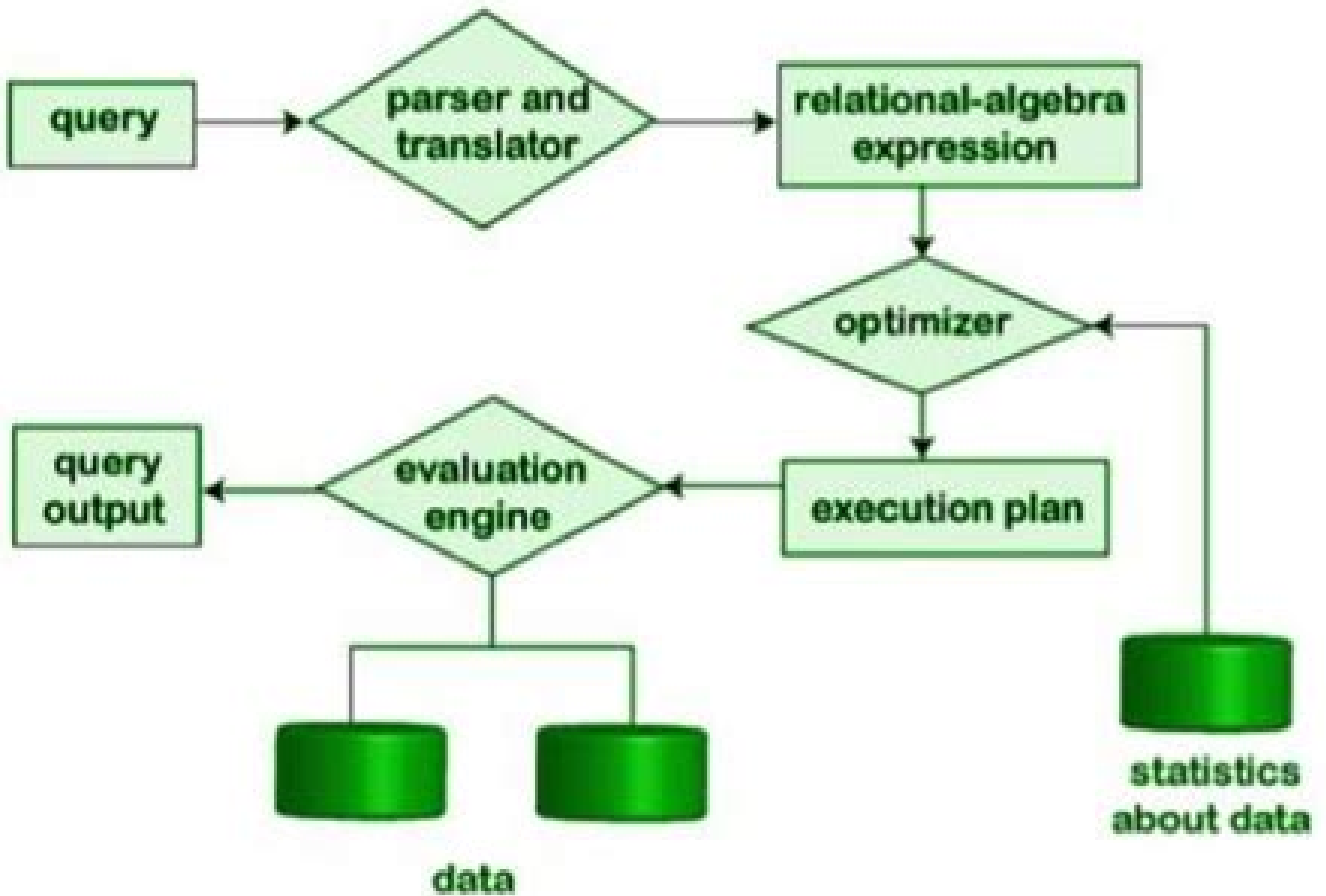
Steps in query processing
