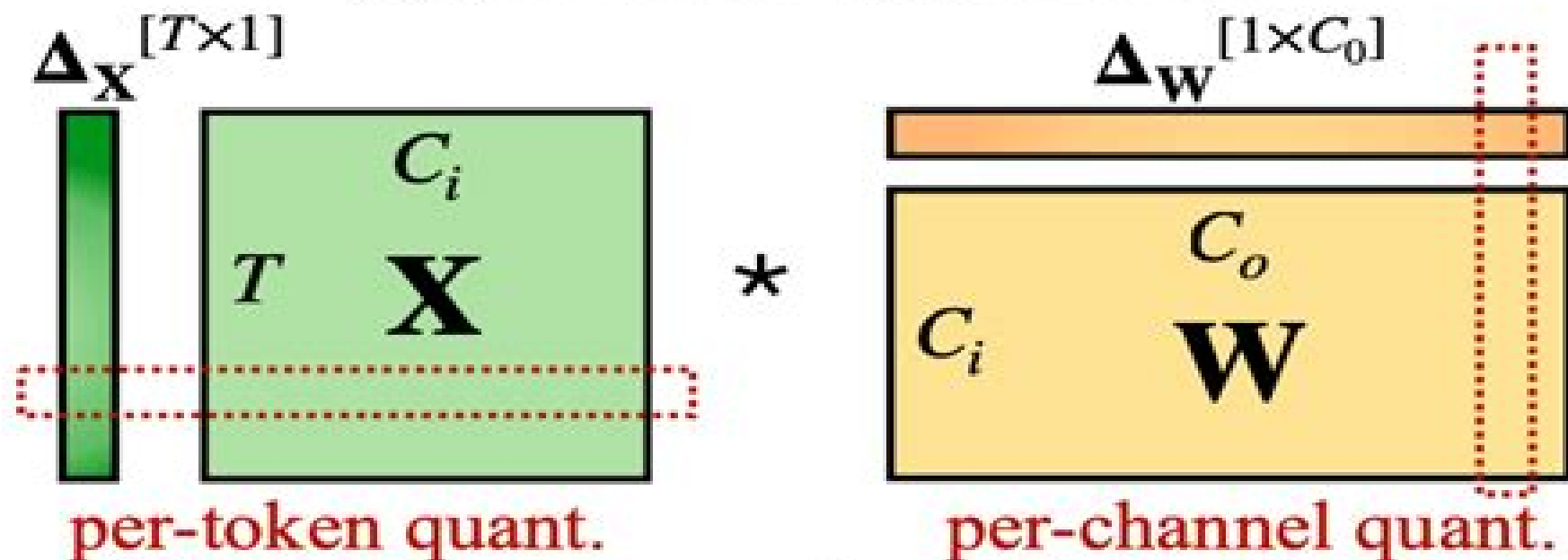
(b) per-token + per-channel quantization
