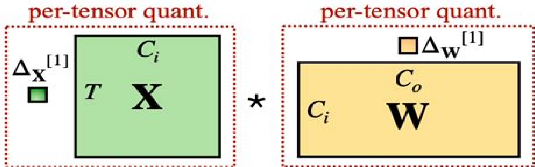
(a) per-tensor quantization
