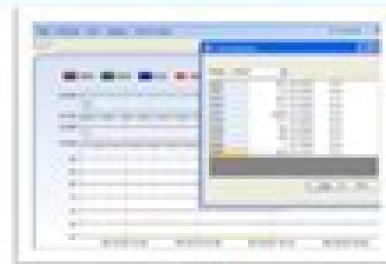
ANACON Software
