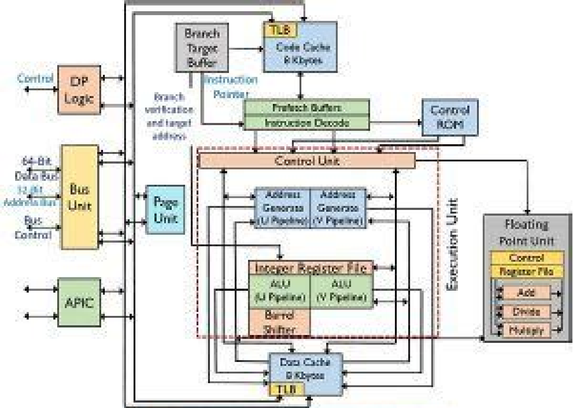
Architecture of Pentium Processor
